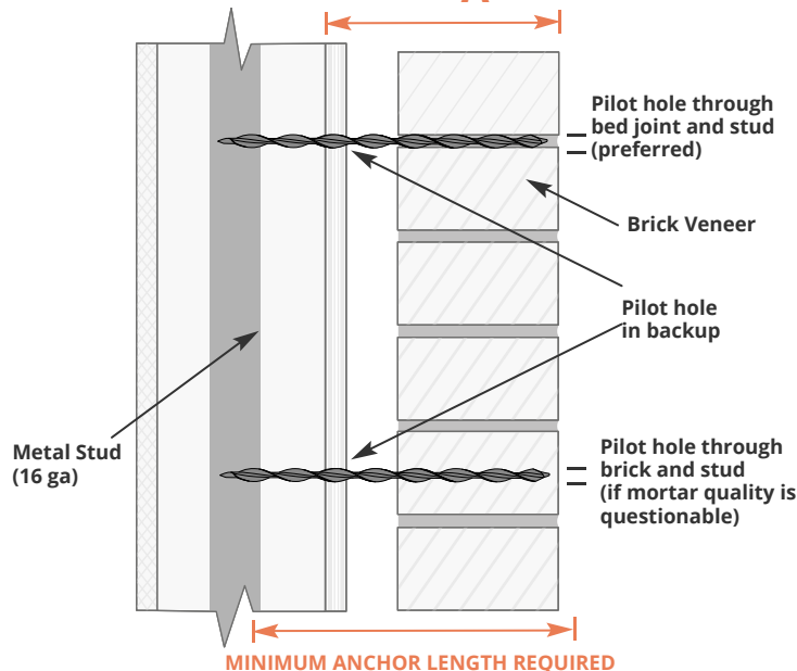
Section view
