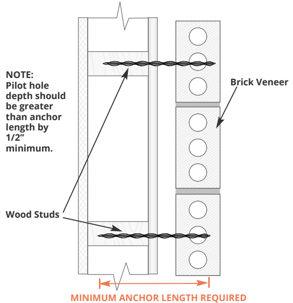
Plan view
