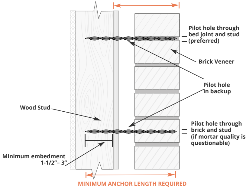
Section view
