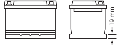
B4 Base hold-down 19 mm (on long sides)
