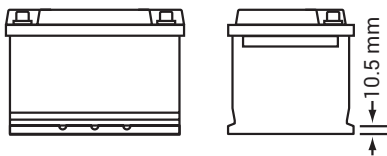
B1 Base hold-down 10.5 mm (on long sides)
